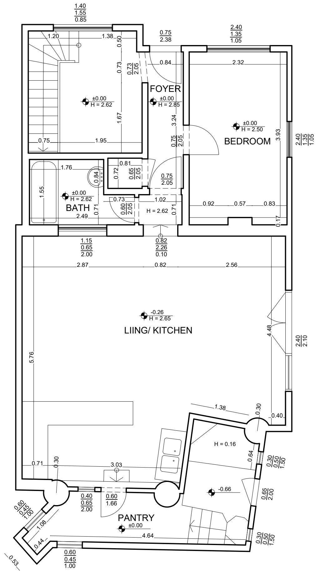
GROSS INTERNAL AREA FLOOR 1: 70.81 SQM
